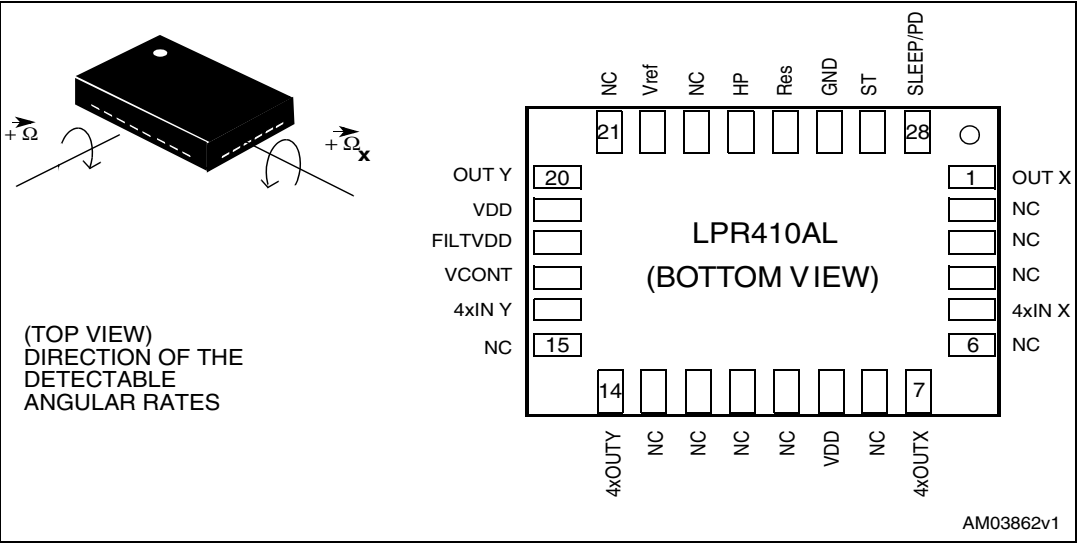
Figure 2. Pin connection
