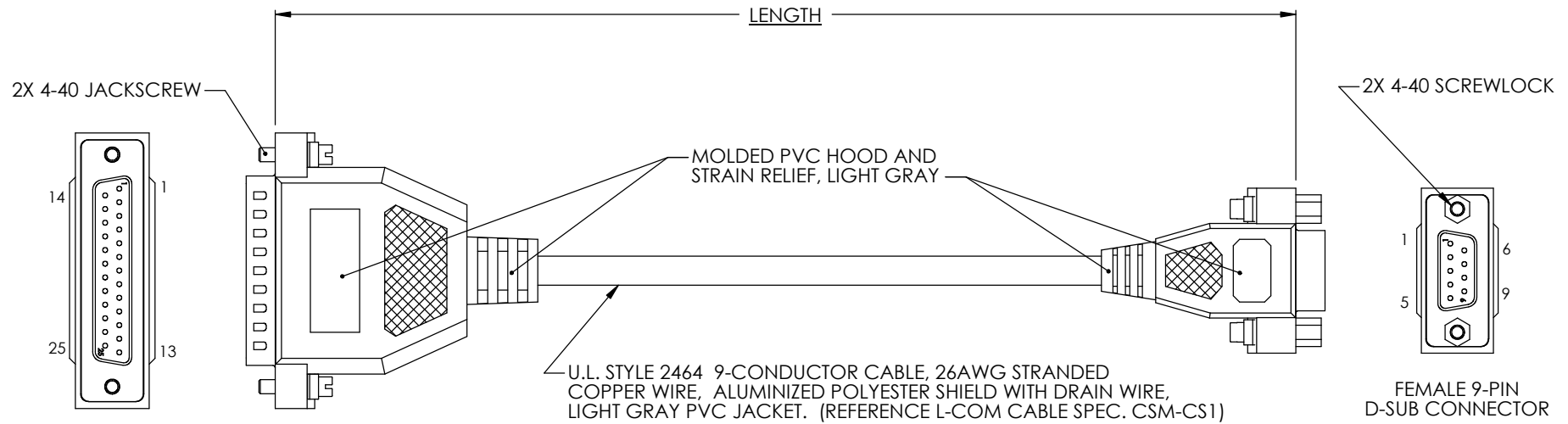
MALE 25-PIN D-SUB CONNECTOR
