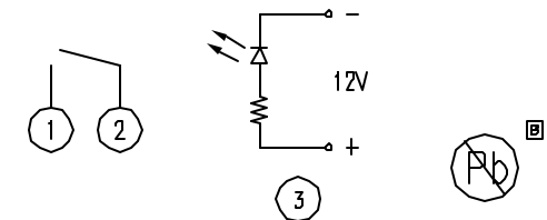
INTERNAL CIRCUIT
