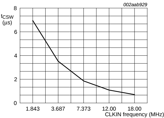
Fig 22. t CSW as a function of CLKIN frequency
