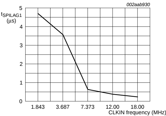
Fig 23. t SPILAG1 as a function of CLKIN frequency
