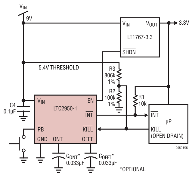
Figure 5. Input Voltage Monitoring with \overline{\text{KILL}} Input
