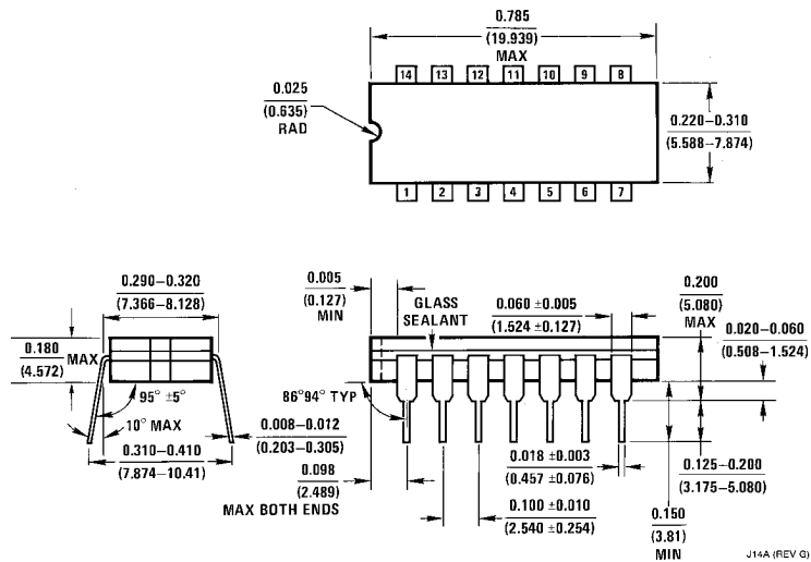
14-Lead Ceramic Dual-In-Line Package (J) Order Number 54LS125ADMQB or DM54LS125AJ Package Number J14A
