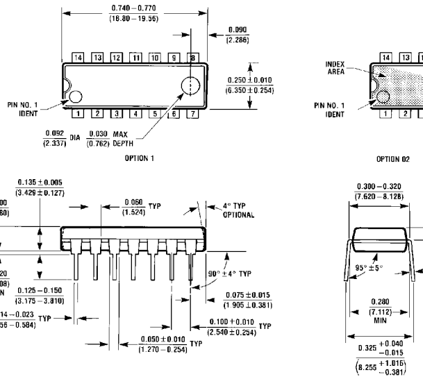
14-Lead Molded Dual-In-Line Package (N) Order Number DM74LS125AN Package Number N14A
