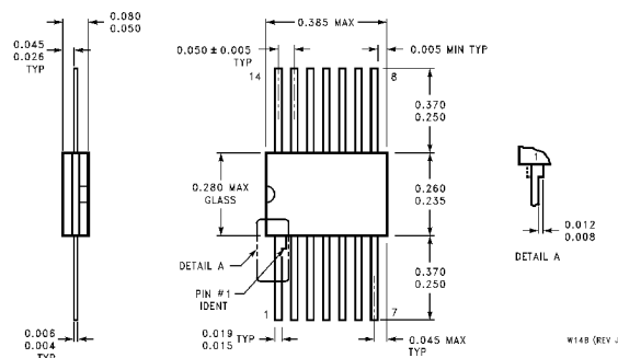
14-Lead Ceramic Flat Package (W) Order Number 54LS125AFMQB or DM54LS125AW Package Number W14B
