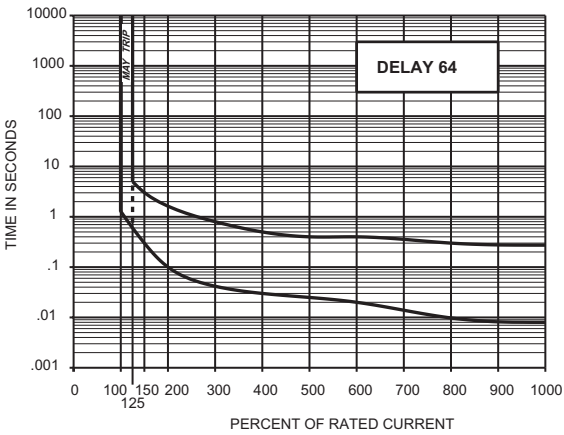
60Hz Delay Curves (typ)
