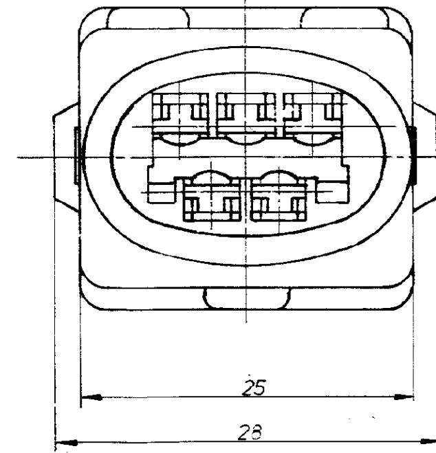
Ansicht VIEW "X"
