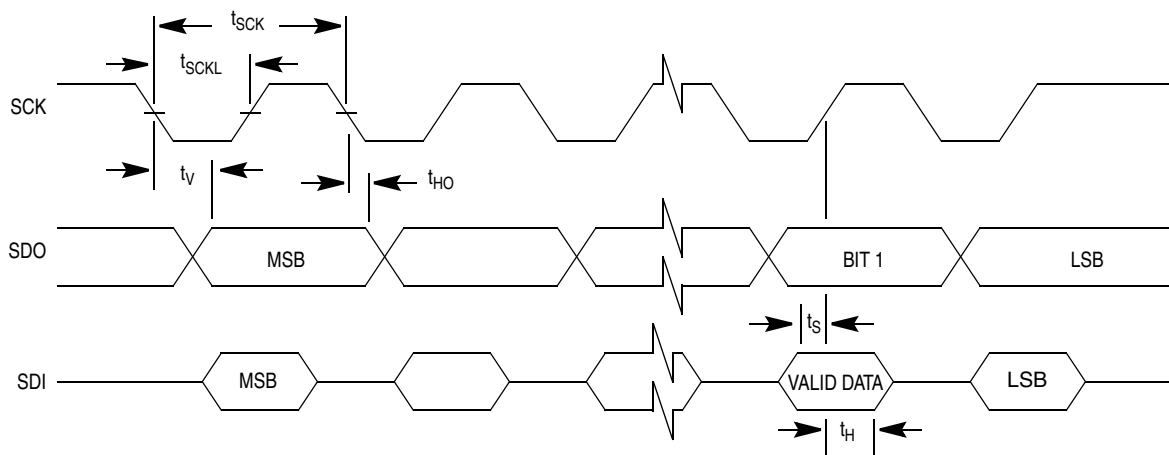
Figure 15-11. SIOPTiming Diagram
