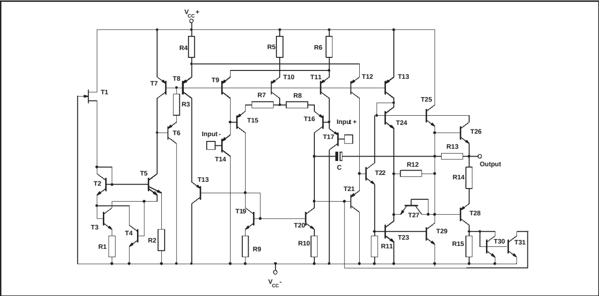
SCHEMATIC DIAGRAM (for 1/4 MC33174)
