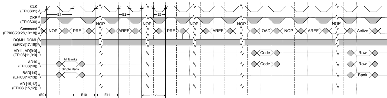
Figure 24-10. SDRAM Initialization and Load Mode Register Timing
