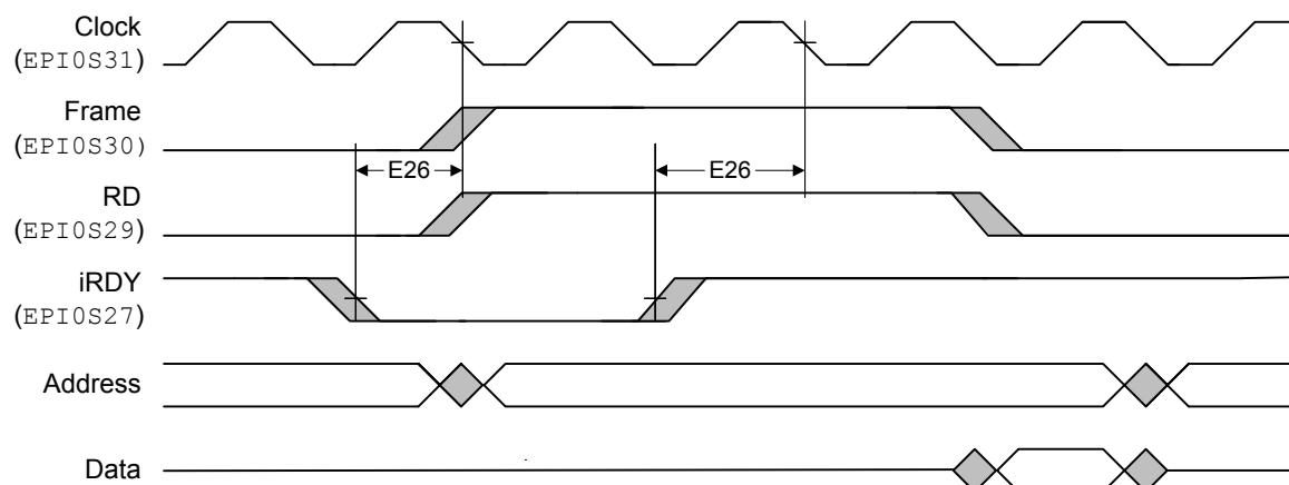
Figure 24-16. General-Purpose Mode iRDY Timing
