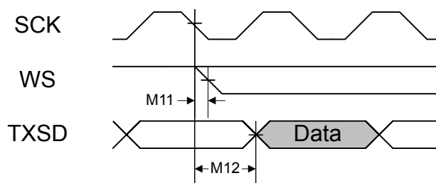
Figure 24-22. I 2 S Master Mode Transmit Timing
