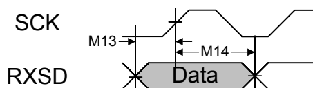
Figure 24-23. I 2 S Master Mode Receive Timing
