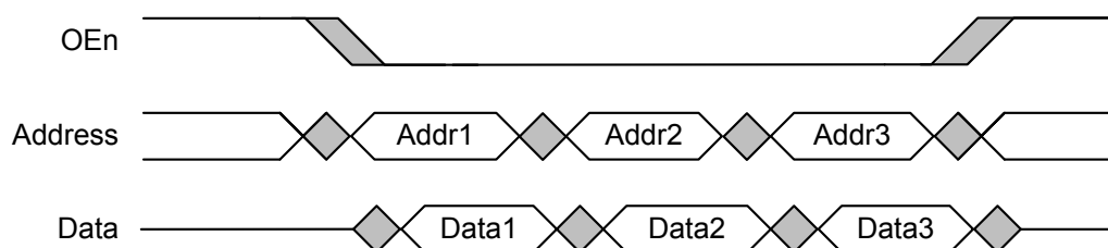
Figure 9-8. Continuous Read Mode Accesses
