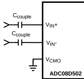
Figure 31. Differential Input Drive
