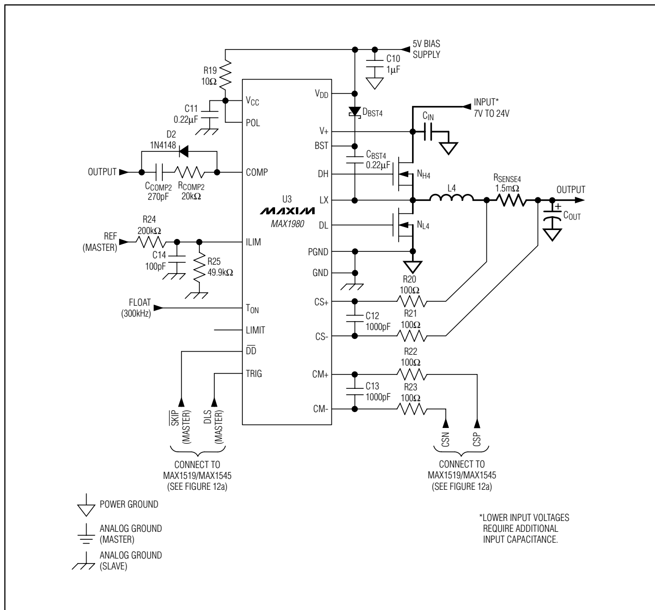
Figure 12c. Standard 4-Phase Desktop 4 Application Circuit (4th Phase—MAX1980 Slave)
