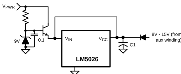
Figure 28. Start-Up Regulator for V_{PWR} > 100V
