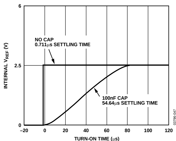
Figure 21. Internal V_{REF} vs. Turn-On Time
