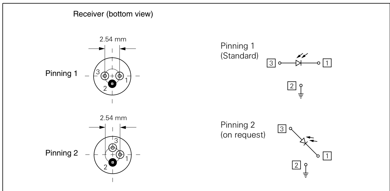
Figure 2 Receiver
