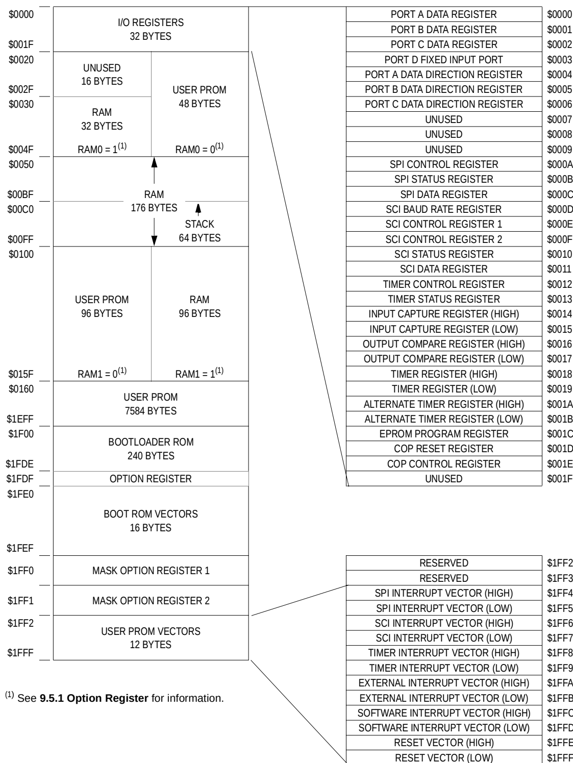
Figure 2-1. Memory Map
