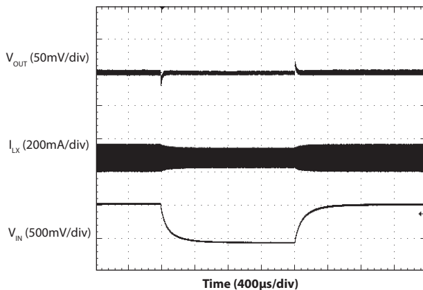
Line Transient Response — PWM
