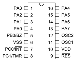
HT48R06A-1 – 16 SSOP
