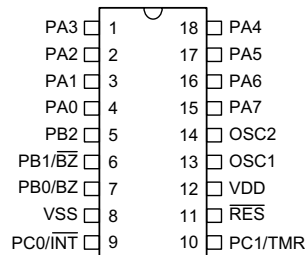
HT48R06A-1 – 18 DIP/SOP
