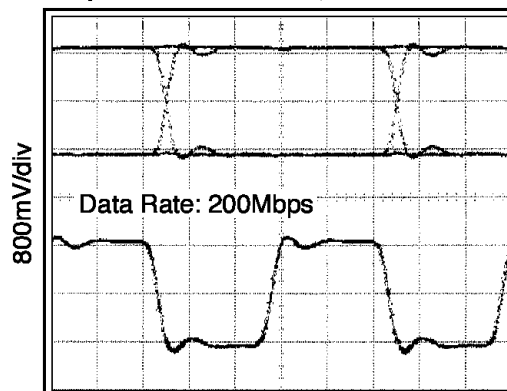
Output Data and Clock, Differential
