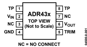
Figure 1. 8-Lead MSOP (RM Suffix)
