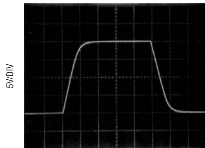
Large Signal Transient Response G = 100, V_S = \pm 15\text{V}
