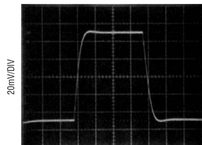
Small Signal Transient Response G = 10, V_S = \pm 15\text{V}
