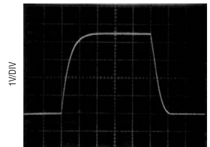
Large Signal Transient Response G = 100, V_S = 5\text{V}, 0\text{V}
