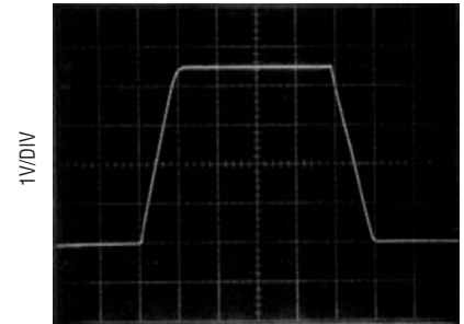
Large Signal Transient Response G = 10, V_S = 5\text{V}, 0\text{V}
