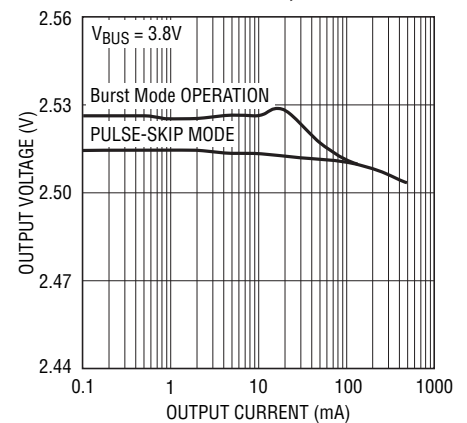
Switching Regulators 1, 2 Load Regulation at V_{OUT1,2} = 2.5\text{V}
