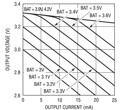
3.3V LDO Output Voltage vs Output Current, V_{BUS} = 0V
