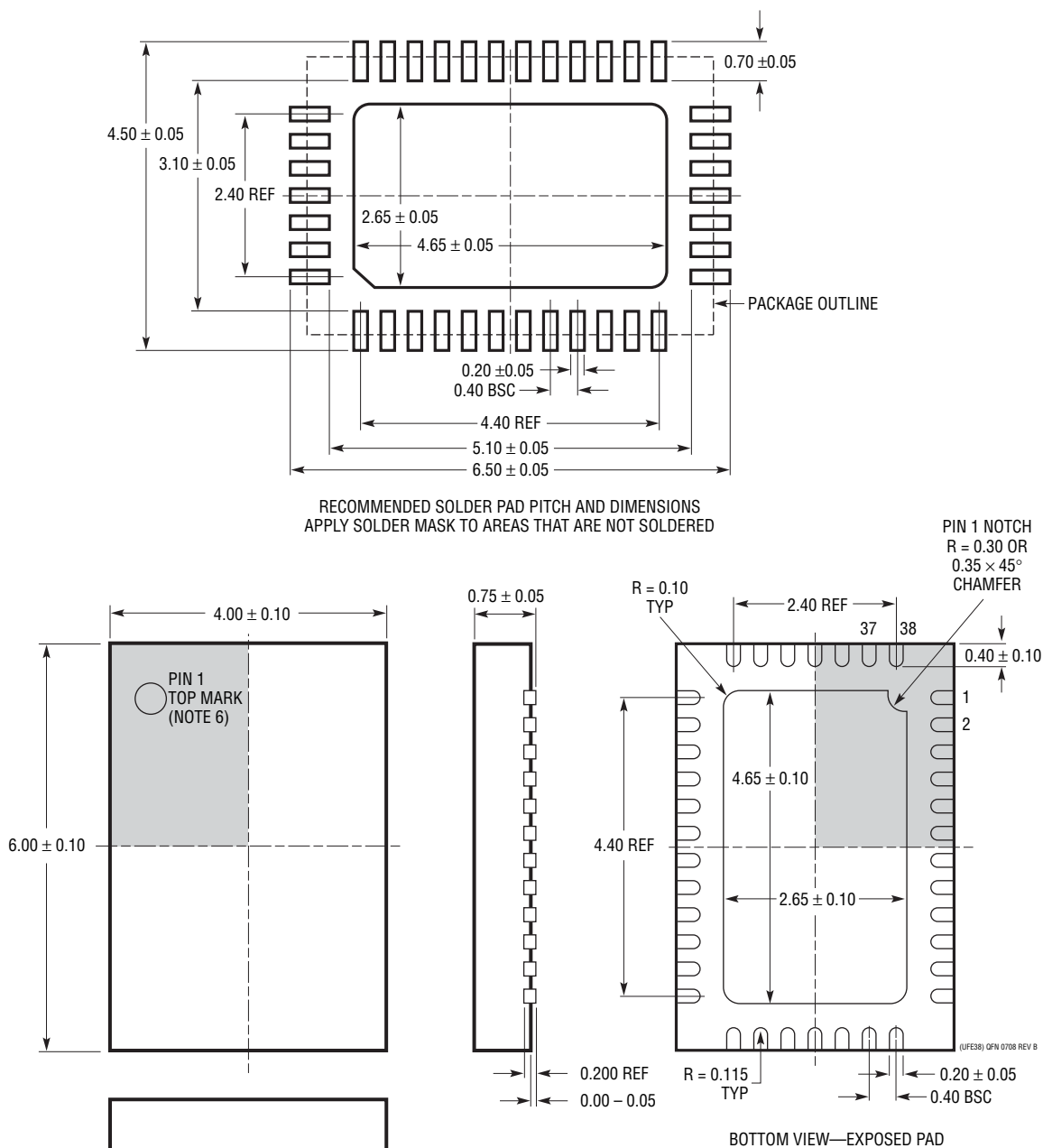
UFE Package 38-Lead Plastic QFN (4mm × 6mm) (Reference LTC DWG # 05-08-1712 Rev B)
