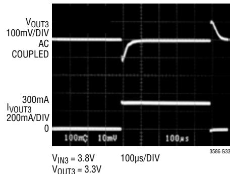
Buck-Boost Step Response
