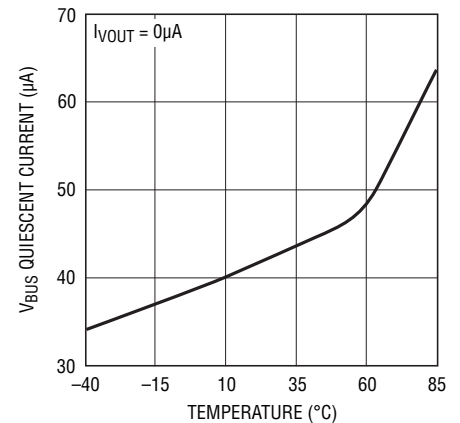
V_{\text{BUS}} Quiescent Current in Suspend vs Temperature
