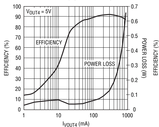
Boost Efficiency ( V_{IN4} = 3.8\text{V} )
