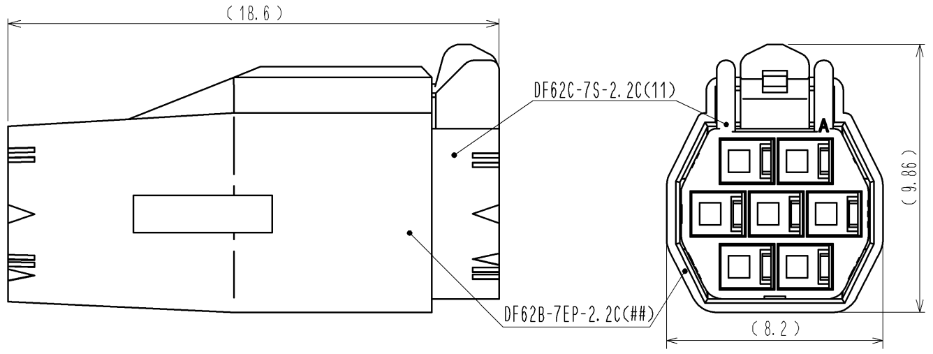
MATING FIGURE
