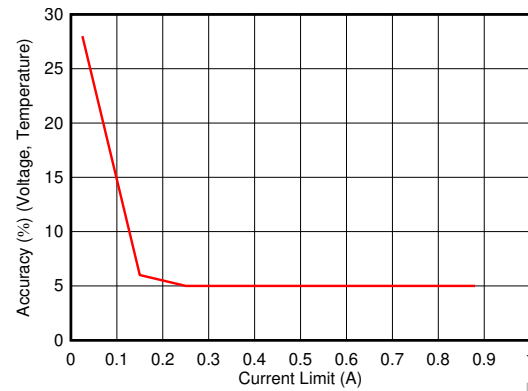
Figure 7-20. Current Limit Accuracy vs Current Limit, I_{\text{OL}}
