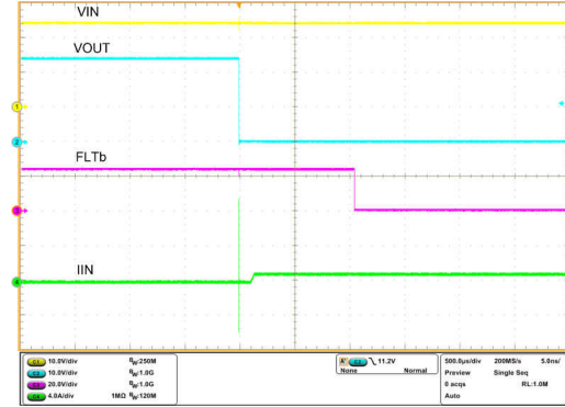
R_{ILIM} = 7.5 \text{ k}\Omega R_{FLTb} = 100 \text{ k}\Omega Figure 7-26. Hot-Short: Fast-Trip Response and Current Regulation
