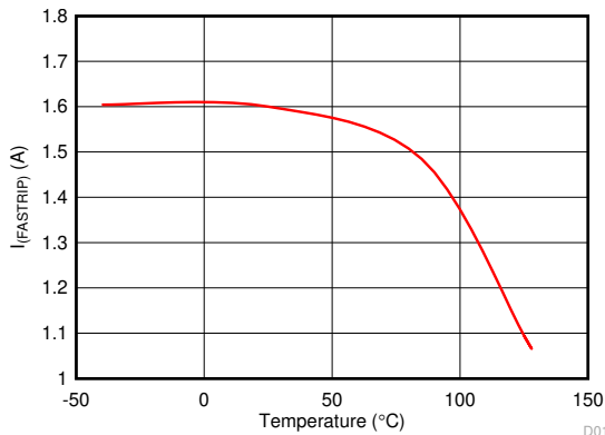
Figure 7-19. Fast-Trip Comparator Threshold I_{\text{FAST-TRIP}} vs Temperature Threshold
