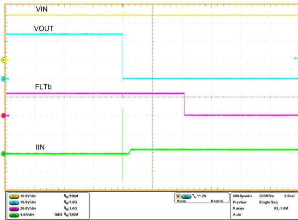
Figure 9-10. Output Hot Short Functionality at 24-V Input
