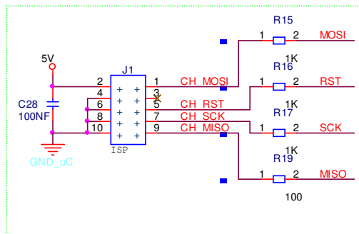
Figure 11: Microcontroller programming
