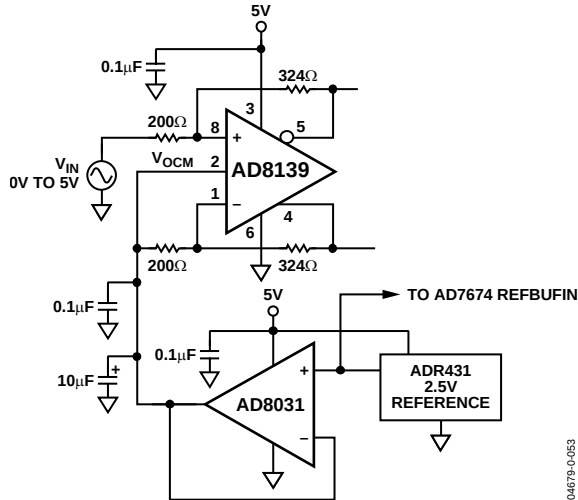
Figure 60. Low-Z 2.5 V Buffer
