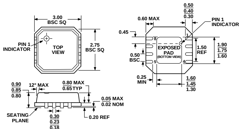
Figure 64. 8-Lead Lead Frame Chip Scale Package [LFCS], 3 mm x 3 mm Body (CP-8-2)—Dimensions shown in millimeters
