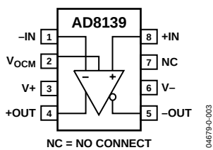
Figure 4. Pin Configuration
