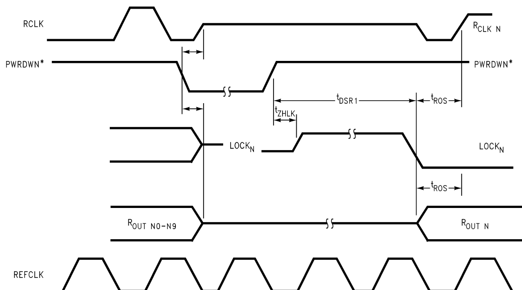
Figure 4. Locktime from PWRDN* t_{DS1}
