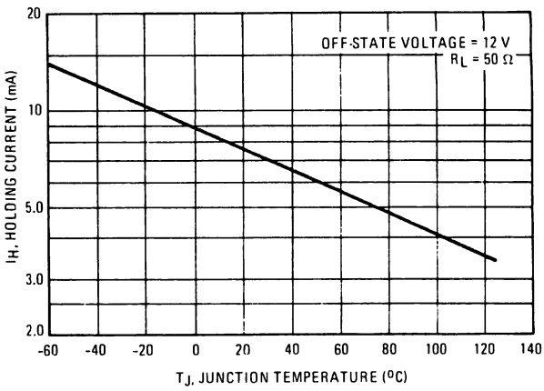
FIGURE 9 – HOLDING CURRENT
