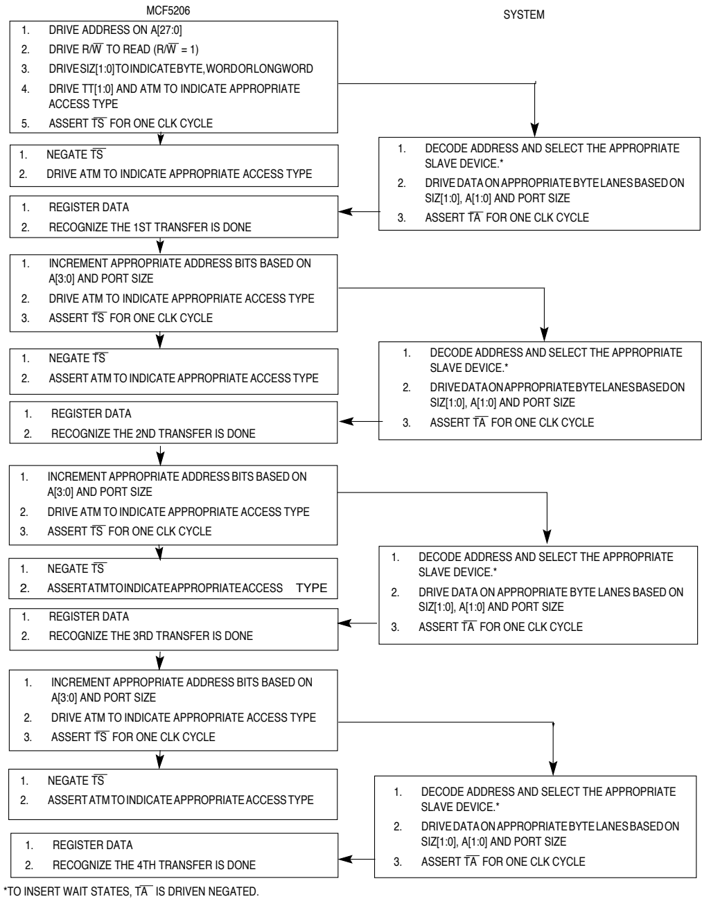
Figure 3-12. Burst-Inhibited Word-, Longword-, and Line-Read Transfer Flowchart
