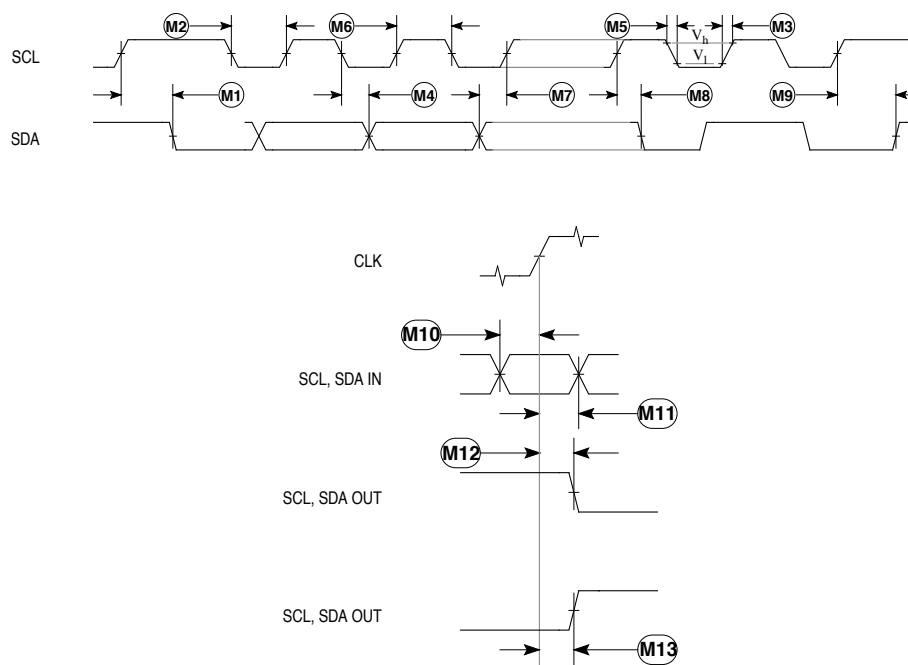
M-Bus Timing
