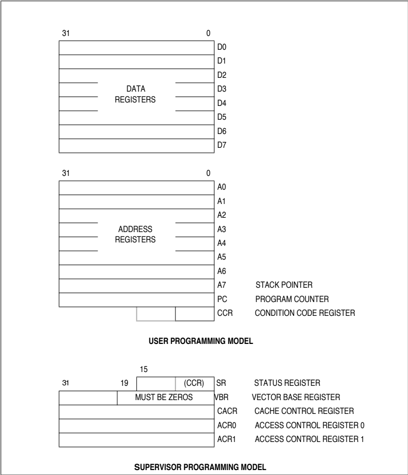
Figure 1-2. Programming Model
