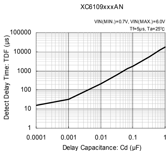
(9) Detect Delay Time vs. Delay Capacitance
