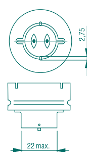
BY 22d
