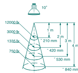
Hi-Spot ESD111 100W / 10°
