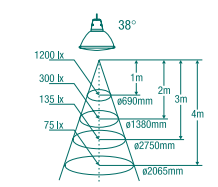
Coolfit 50W / 38°
