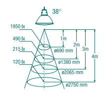
Coolfit 35W / 38°
