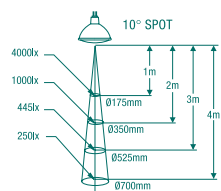
Superia 50 / 20W / 10°
