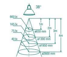
Coolfit 20W / 38°
