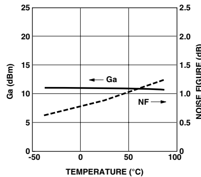
Figure 15. AT-31033 Noise Figure and Associated Gain at V_{CE} = 2.7 V, I_C = 1 mA vs. Temperature in Test Circuit, Figure 1. (Circuit Losses De-embedded)
