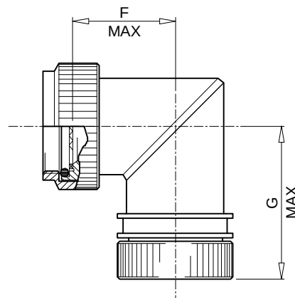
90° ADAPTOR
