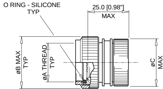
STRAIGHT ADAPTOR
