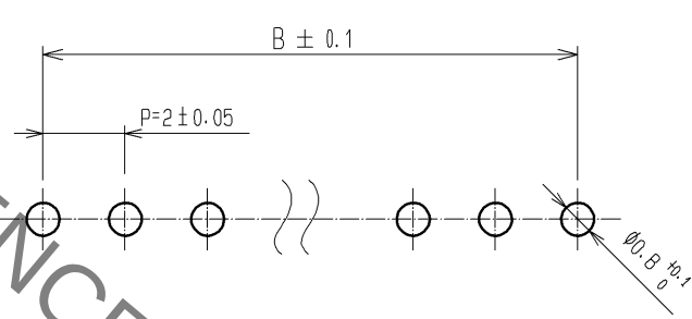
RECOMMENDED PATTERN(BOARD THICKNESS t=1.6mm)
