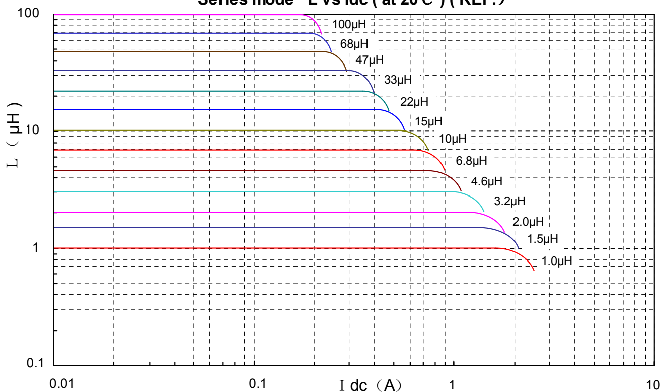
Series mode L vs I dc ( at 20℃ ) ( REF. )
