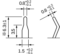
(Terminal dimensions)
