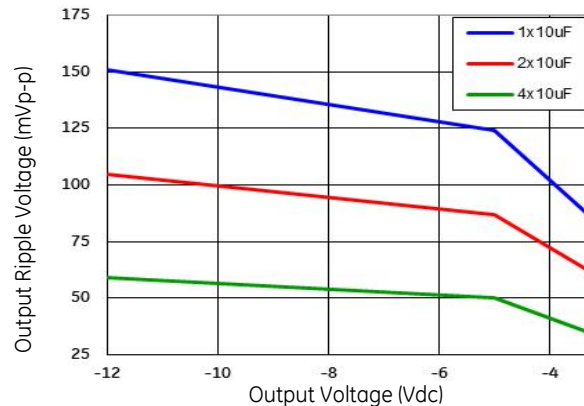
Figure 64. Output ripple with 1x10 \mu F, 2x10 \mu F & 4x10 \mu F output ceramic capacitors (max load).
