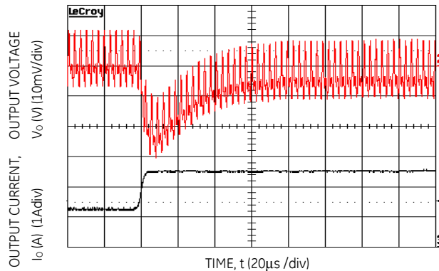
Figure 10. Transient Response to Dynamic Load Change from 50% to 100% at 28Vin, C_{ext} = 10\mu F ceramic + 330 \mu F polymer, C_{Tune} = 5600pF & R_{Tune} = 261\Omega
