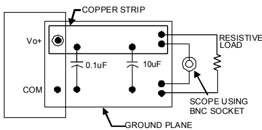
Figure 25. Input Reflected Ripple Current Test Setup.
