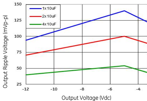
Figure 62. Output ripple with 1x10 \mu F, 2x10 \mu F & 4x10 \mu F output ceramic capacitors (max load).
