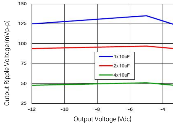
Figure 63. Output ripple with 1x10 \mu F, 2x10 \mu F & 4x10 \mu F output ceramic capacitors (max load).
