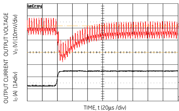
Figure 4. Transient Response to Dynamic Load Change from 50% to 100% at 28Vin, C ext = 10μF ceramic + 330μF polymer, C Tune =5600pF & R Tune =261Ω
