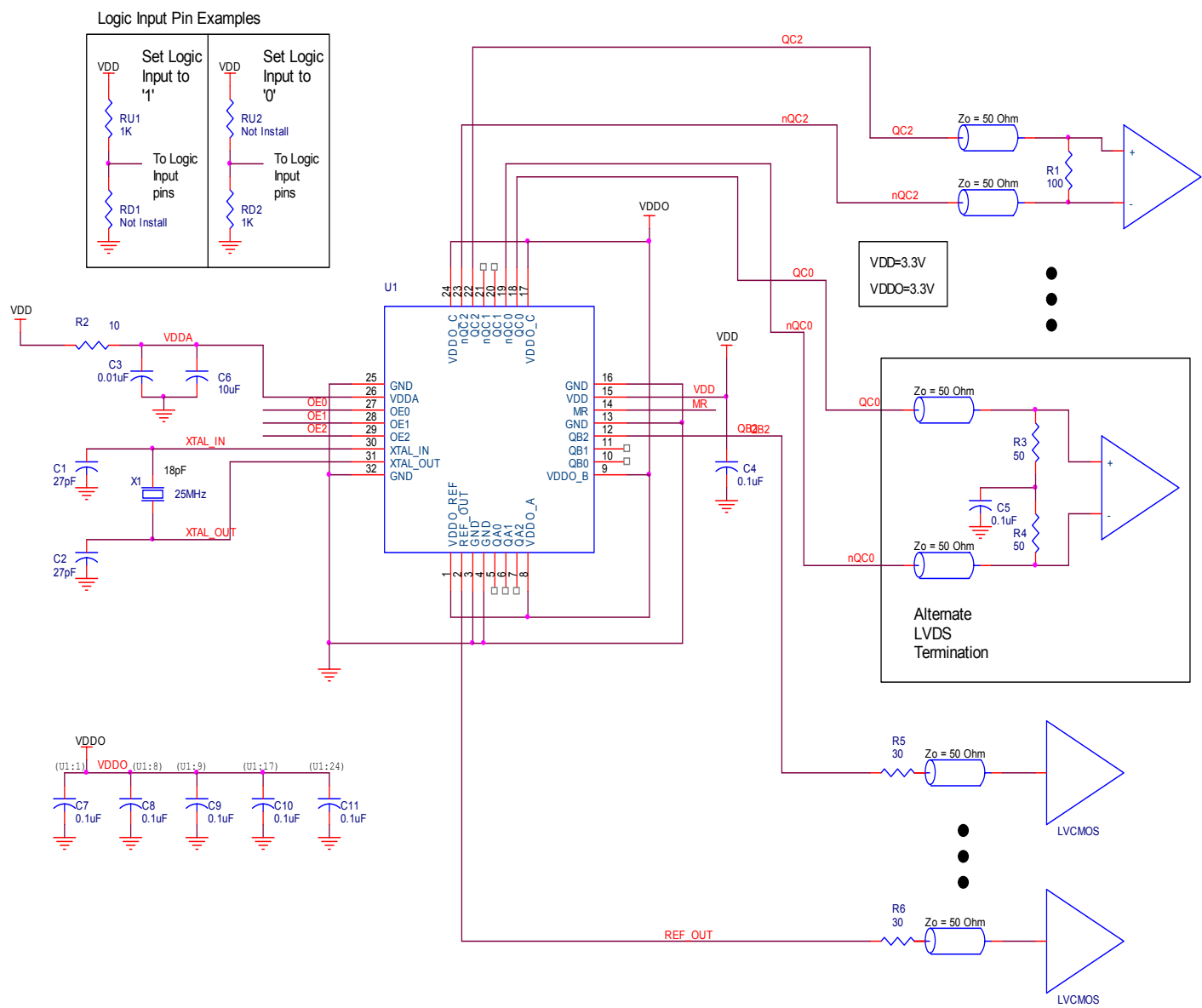
Figure 6. ICS8402015I Schematic Example
