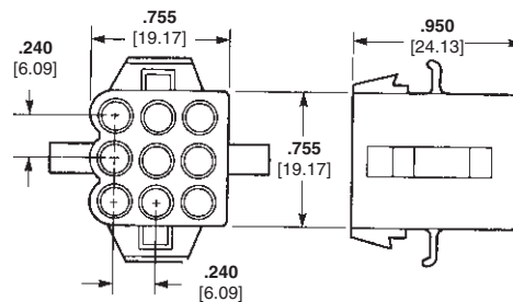
Socket Housing (Plug)
