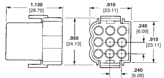
Pin Housing (Cap)
