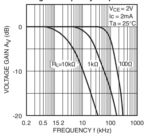
Fig. 14 Frequency Response
