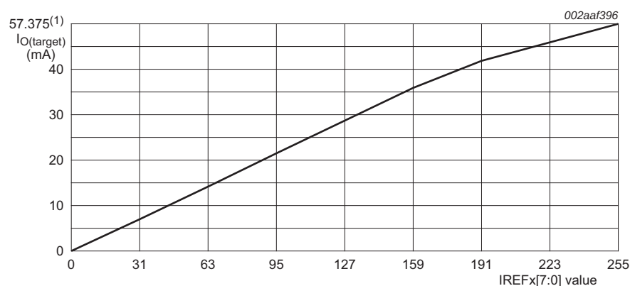
Fig 6. I_{\text{O(target)}} versus IREFx value
