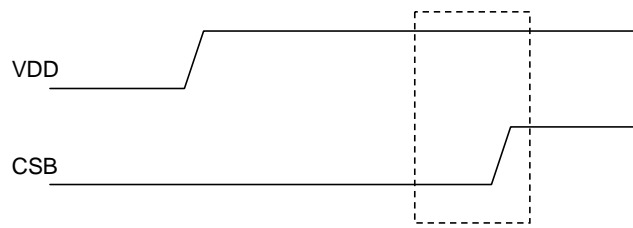
Figure 32. CSB Timing
