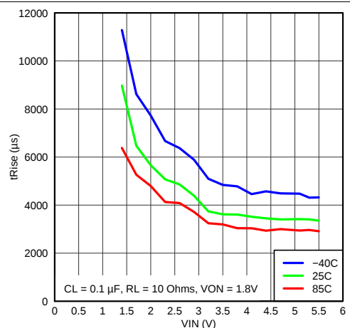
Figure 19. Rise Time vs Input Voltage
