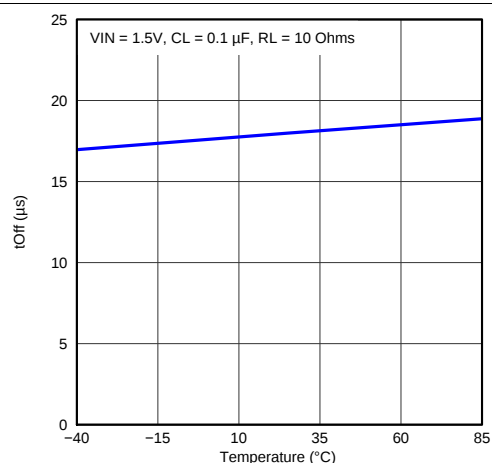
Figure 17. Turn-Off Time vs Temperature
