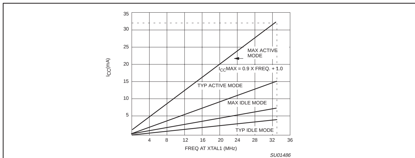
Figure 34. I_{CC} vs. FREQ for 12-clock operation
