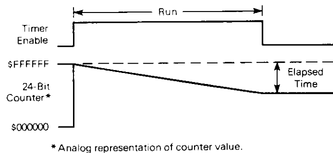
Figure 5-4. Elapsed Time Measurement Example
