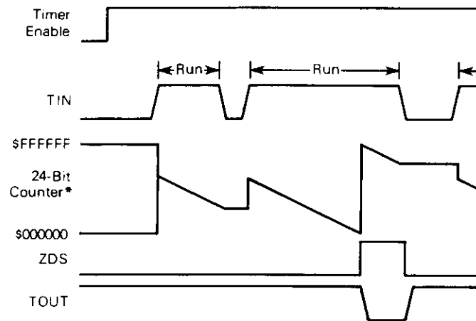
Figure 5-5. Device Watchdog Example
