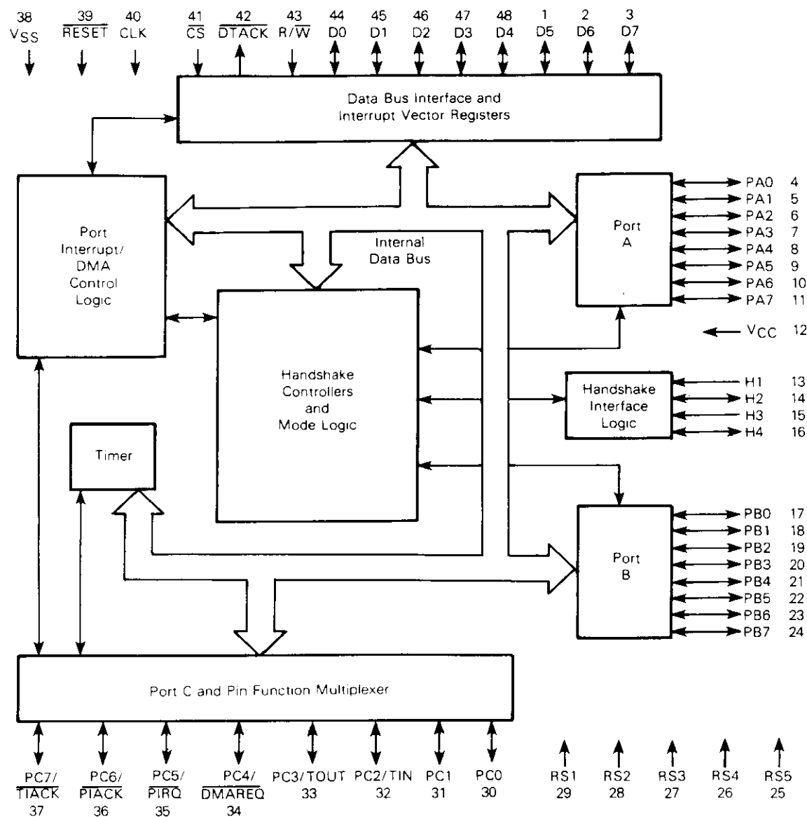
Figure 1-1. Block Diagram
