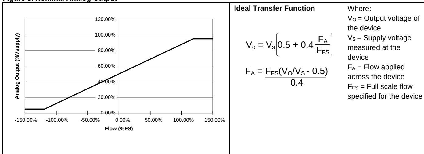
Figure 3. Nominal Analog Output
