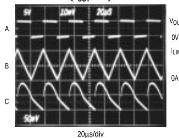
MEDIUM-LOAD SWITCHING WAVEFORMS ( V_{OUT} = 5V )
