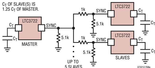
Figure 8a. SYNC Output (Master Mode)
