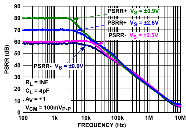
FIGURE 7. PSRR vs FREQUENCY, V_S = \pm 0.9V , \pm 2.5V
